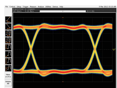
10 Gbps eye captured with 30 GHz of bandwidth
