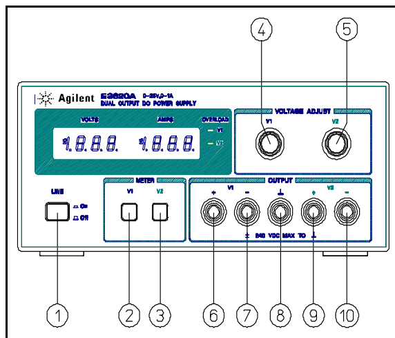
Figure 2. Front-Panel Controls and Indicators
